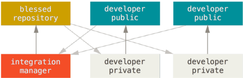
FIGURE 5-2 Integration-manager workflow.
