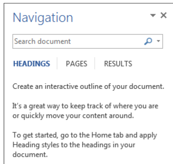
Figure 9 – Navigation Pane
