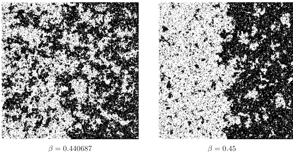
Figure 13.1: The Ising model with Dobrushin boundary conditions (black on the right side of the box and white on the left), at the critical and a slightly supercritical inverse temperature.
