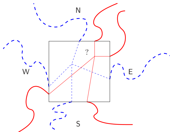
Figure 12.9: Zhang's argument for the impossibility of \theta(1/2) > 0 .
