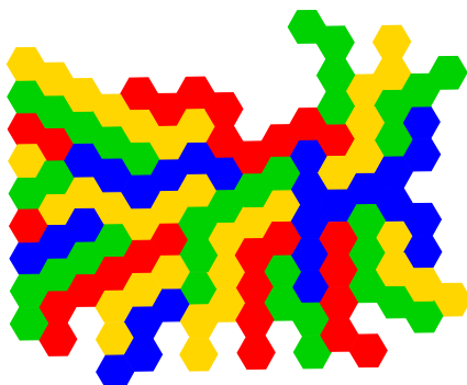
Figure 5.1: Trying to create at least 7 neighbours for each country. It works fine for a while, but then we seem to run out of space.
