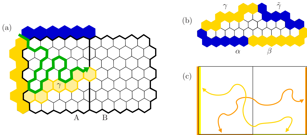
Figure 12.8: Smirnov’s proof of RSW. Open/white denoted by yellow, closed/black denoted by blue. {f.RSW}
