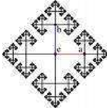
Figure 2.1: The Cayley graph of F_2 .
