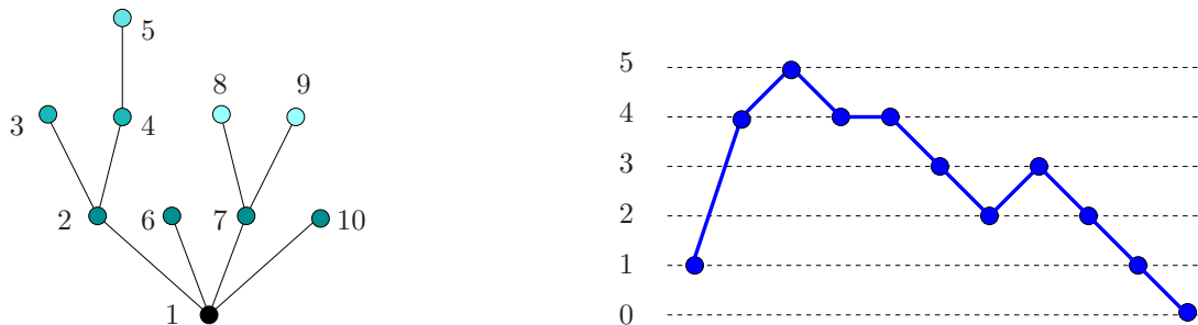
Figure 12.3: On the left, the shades of vertex colours show the order in which the sets of children are put into the active list. The labels on the vertices show the order in which they turn inactive. On the right, the steps of the walk are indexed by the vertices as they turn inactive, while the height shows the current number of active vertices.
