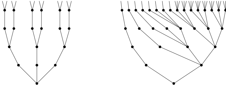
Figure 12.4: A quasi-transitive tree and the 3-1 tree.
