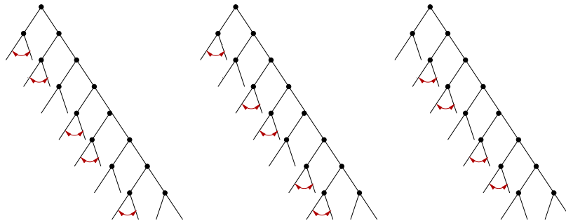
Figure 15.2: The profiles of the generators b, c, d in Grigorchuk’s group.
