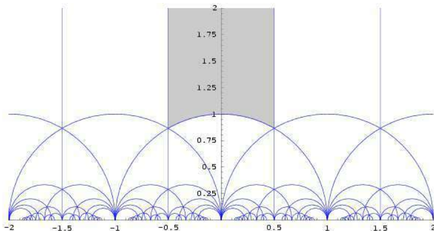
Figure 3.1: A fundamental domain of the action of the modular group \mathrm{PSL}_2(\mathbb{Z}) on \mathbb{H}^2 . Picture by Froppuff (from en wikipedia) [GFDL ( www.gnu.org/copyleft/fdl.html ) or CC-BY-SA-3.0 ( http://creativecommons.org/licenses/by-sa/3.0/ )], via Wikimedia Commons.
