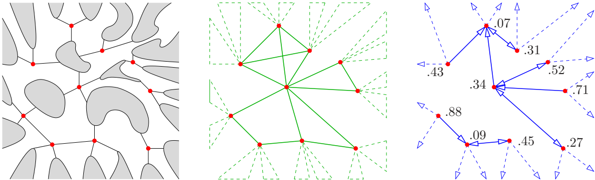
Figure 12.5: Constructing the graph \mathcal{G} and forest \mathcal{F} of trifurcation points in an infinite cluster.
