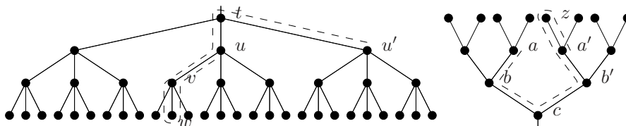
Figure 5.2: The Diestel-Leader graph \text{DL}(3, 2) . A sample path: (u, a) , (v, b) , (w, c) , (v, b') , (u, a') , (t, z) , (u', a') .
