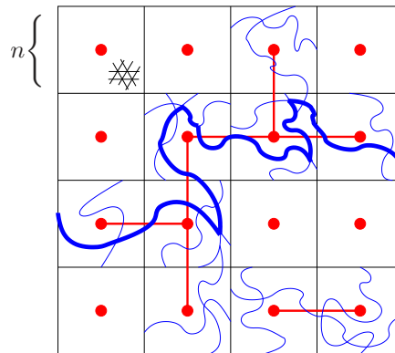
Figure 12.11: Supercritical renormalization: bond percolation on the grid \mathbf{G}_n of n -boxes. \{\mathbf{f. renorm}\}
