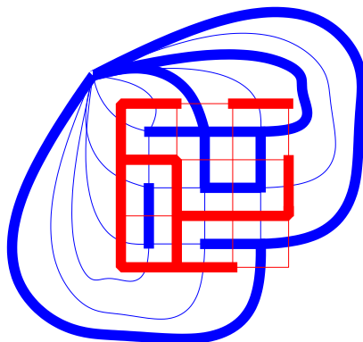
Figure 13.2: The planar dual of an FK configuration on \mathbb{Z}^2 .
