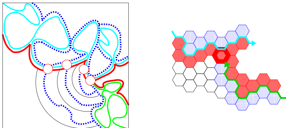
Figure 12.10: Producing c \log n pivots in an n -box with positive probability.
