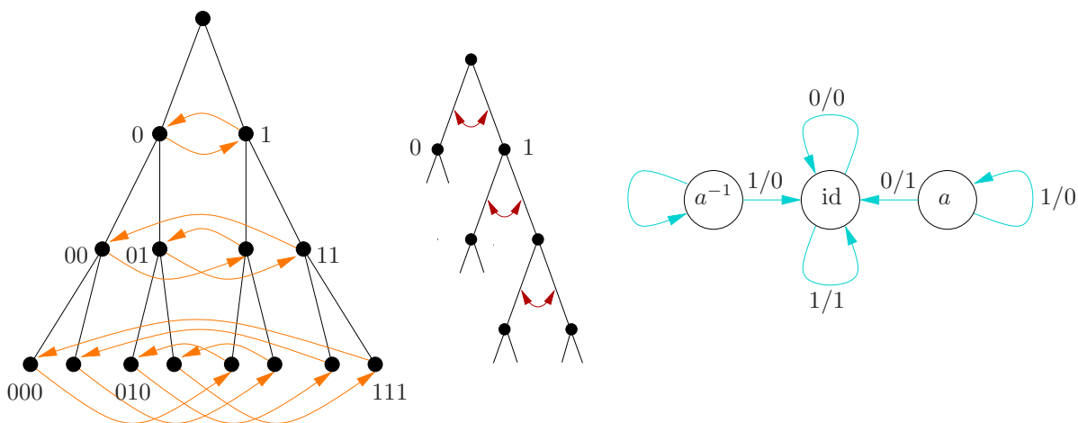
Figure 15.1: The adding machine action of \mathbb{Z} : (a) the Schreier graphs on the levels (b) the profile of the generator a ’s action (c) the Moore diagram of the automaton
