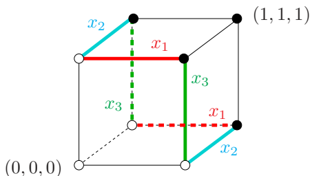
Figure 12.6: For majority on 3 variables, \mathcal{A} = \text{Maj}_3 := \{x \in \{0, 1\}^3 : \sum_{i=1}^3 x_i \geq 2\} , each variable is pivotal in four configurations (at the endpoints of two edges).
