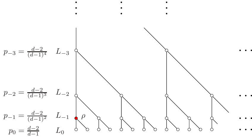
Figure 14.1: The “canopy tree” T_d^* with a random root \rho (now on level L_{-1} ), which is the local weak limit of the balls in the d -regular tree \mathbb{T}_d , for d = 3 .
