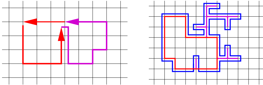
Figure 2.2: (a) Combining two loops. (b) Homotopic loops inside \mathbb{Z}^2 .
