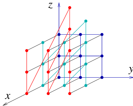
Figure 4.1: The Cayley graph of the Heisenberg group with generators X, Y, Z .
