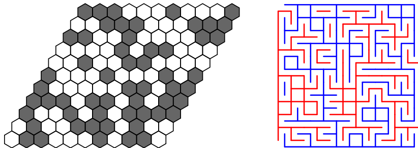
Figure 12.7: The self-duality of percolation on TG and \mathbb{Z}^2 .
