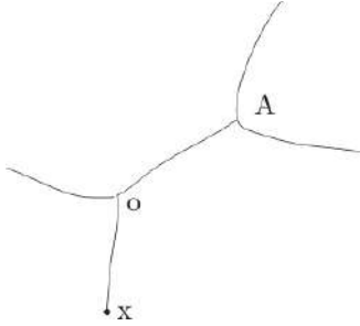
Figure 9.2: Portion of a d -regular tree ( d = 3 )
