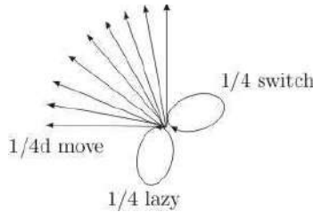
Figure 9.1: The generators for the walk on \mathbb{Z}_2 \wr \mathbb{Z}^d .
