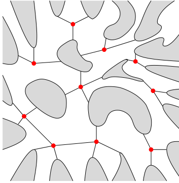
Figure 12.2: Furcation points in an infinite cluster.
