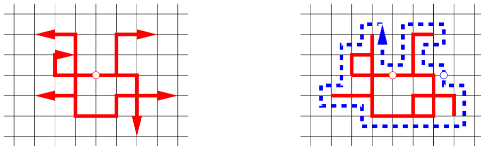
Figure 12.1: Counting primal self-avoiding paths and dual circuits.
